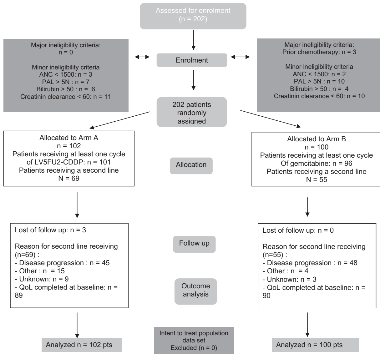
Fig. 1 – Consort diagram.
